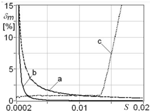
Fig. 5. Maximum converter errors \delta_m vs. S for sinusoidal input voltage, for U_0 = 30 V, U_m = 10 V, f_s = 0,002 f_{s\text{amp}} ; pulse instant calculated from: a – last voltage sample (5), b – two last voltage samples (6), c – mean value of voltage samples after last pulse (8)
