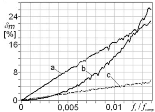
Fig. 4. Maximum converter errors \delta_m vs. signal frequency to sampling frequency ratio for sinusoidal input voltage, for U_0 = 30 V, U_m = 10 V, S = 0,0025 Hz/V; pulse instant calculated from: a – last voltage sample (5), b – two last voltage samples (6), c – mean value of voltage samples after last pulse (8)
