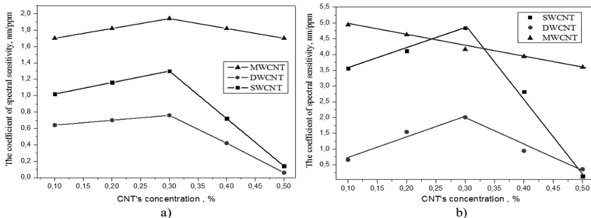
Fig.6. Dependence of the spectral sensitivity of the CNM 5SV concentration of 25% of the concentration of nanotubes on the area from 0 to 30 ppm: a) for short-wave minimum; b) for a double-waved minimum
