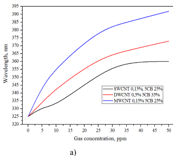
Fig.4. Dependence of change of wavelength of short-wave minimum transmission (a) and long-wave minimum transmission the light (b) from the concentration of SO 2 for CNM with nanotubes
