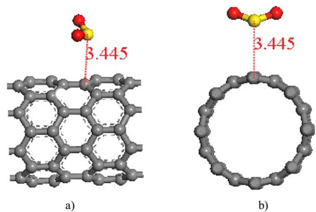
Fig.3. Appearance of the system of carbon nanotube – SO 2 side view (a) and top view (b) [6]
