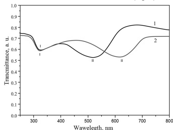
Fig.1. The range of transmission CNM with carbon nanotubes: 1 – 5CB concentration – 25%, 2 – 35% 5CB concentration
