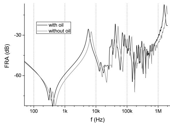
Fig. 7. FR results of transformer with and without oil (autotransformer D)
