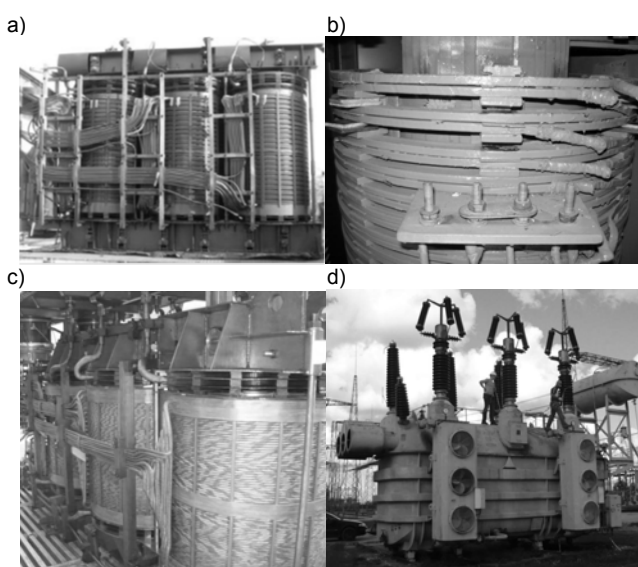
Fig. 1. Transformers used for deformational tests: a) active part of unit A, b) winding with axial deformation of unit B, c) active part of unit C, d) autotransformer D
