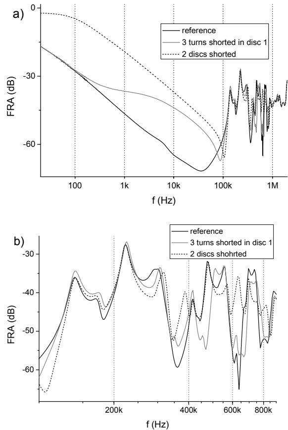
Fig. 6. FR results of short-circuit obtained from transformer B: a) the whole frequency range, b) zoomed range above 100 kHz
