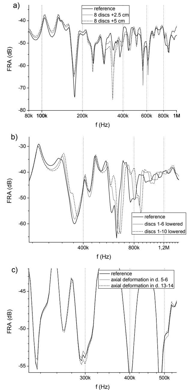
Fig. 3. FR results of axial deformations obtained from transformers A (Fig. 3a), B (Fig. 3b) and D (Fig. 3c)
