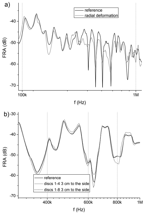
Fig. 4. FR results of radial deformations obtained from transformers A (a) and B (b)
