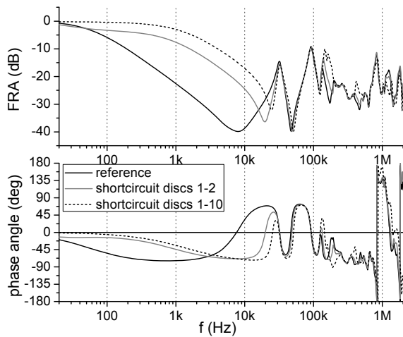
Fig. 5. FR results of short-circuit obtained from transformer C, damping and phase angle
