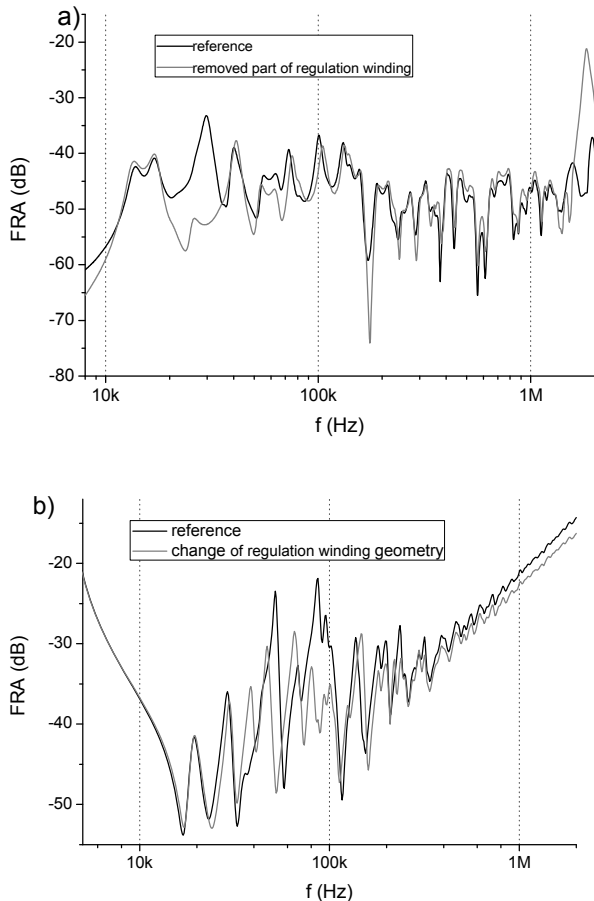
Fig. 2. FR results of rough deformations obtained from transformers A (a) and D (b)
