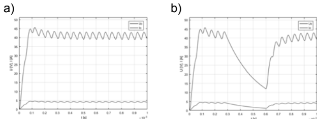
Fig. 11 Output voltage of FORWARD converter: a) without disturbances, b) with disturbances in the clock line.
