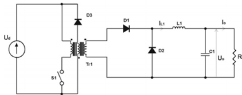
Fig. 4 Diagram of a FORWARD converter.
