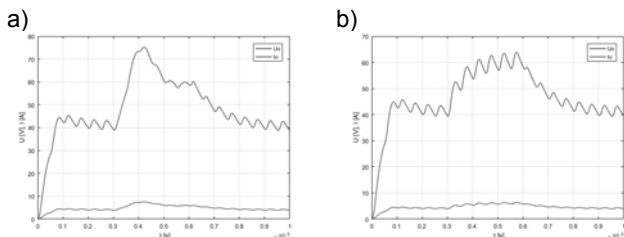
Fig. 14 Output voltage of FORWARD converter with transformer disturbances in: a) winding 1, b) winding 2.
