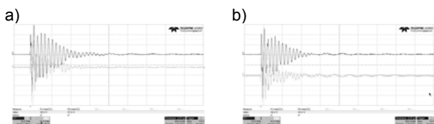
Fig. 24 Converter output voltage with isolated output: a) IN + disturbances, b) OUT + disturbances.
