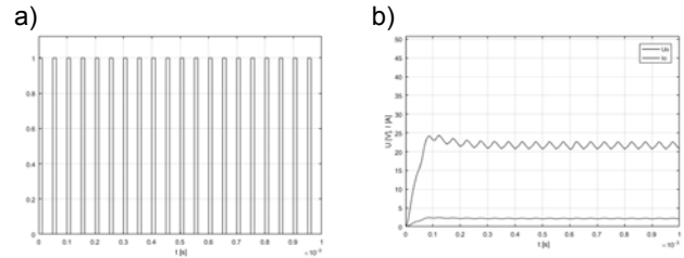
Fig. 6 Converter without disturbances: a) clock signal, b) output voltage.
