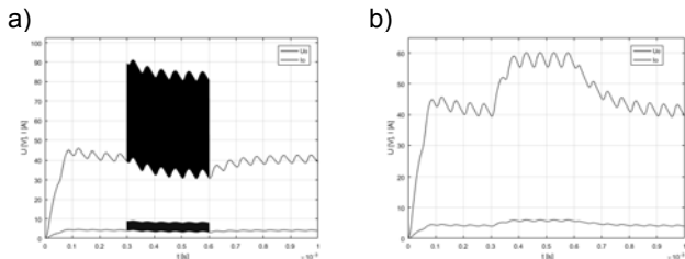
Fig. 12 Output voltage of FORWARD converter: a) with load disturbances R0, b) with L1C1 filter.
