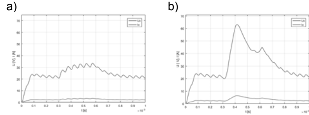
Fig. 9 Converter with disturbances: a) in front of diode D, b) in front of diode D and in clock line.
