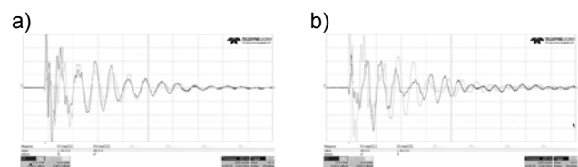
Fig. 18 Universal converter output voltage: a) IN + disturbances, b) OUT + disturbances.
