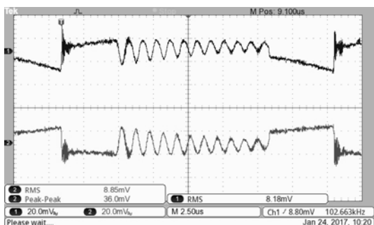
Fig. 20 Voltage reduction converter - work without disturbance.
