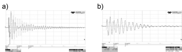
Fig. 21 Voltage reduction converter output voltage: a) IN + disturbances, b) OUT + disturbances.
