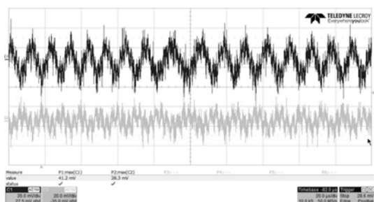
Fig. 23 Converter with isolated output - without disturbances.
