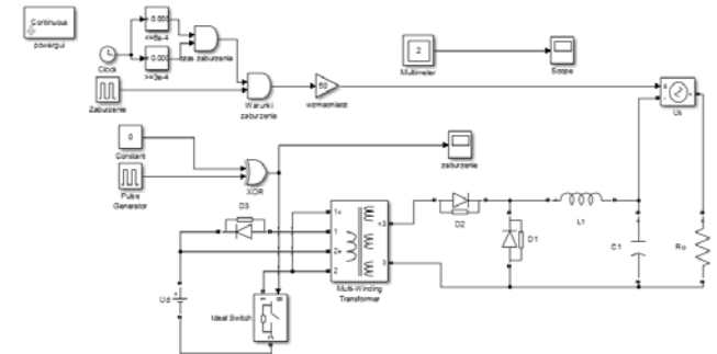
Fig. 10 Numerical model of FORWARD converter.
