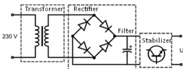
Fig. 1 Linear power supply diagram.
