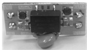
Fig. 22 Converter with isolated output.
