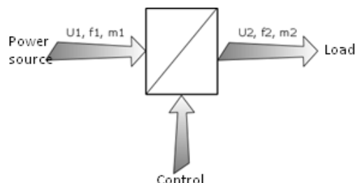
Fig. 2 Block diagram of impulse type power supply.
