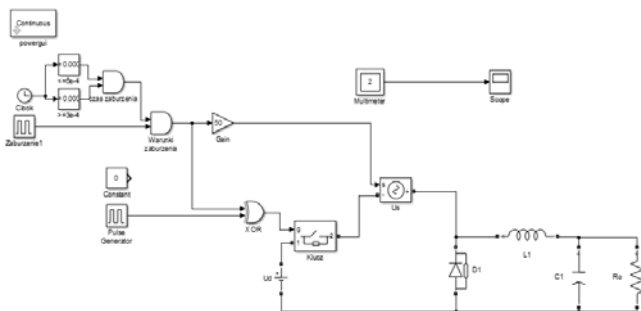
Fig. 5 Numerical model of BUCK type converter
