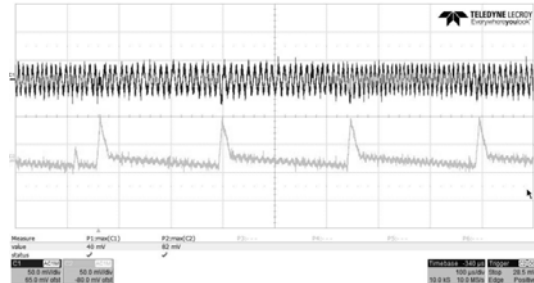
Fig. 17 Input and output voltages of the universal converter at a load current of 25 mA.
