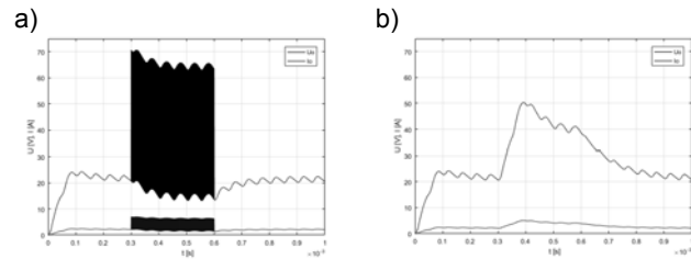
Fig. 8 Converter with disturbances: a) before load R_0 , b) before L_1C_1 filter.
