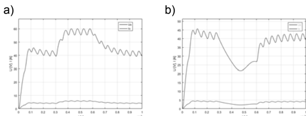
Fig. 13 Output voltage of FORWARD converter: a) with diode D_2 disturbances, b) with diode D_2 disturbance and clock path.
