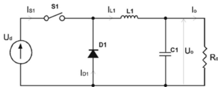
Fig. 3 Diagram of a BUCK converter.
