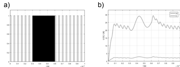
Fig. 7 Converter with clock cycle disturbances: a) clock signal, b) output voltage.
